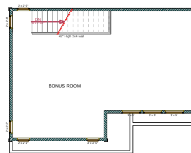
○ UPPER FLOOR PLAN (8'-0 3/4" WALLS) SCALE: 1/4" = 1' - 0" BONUS AREA: 520 Sq Ft
