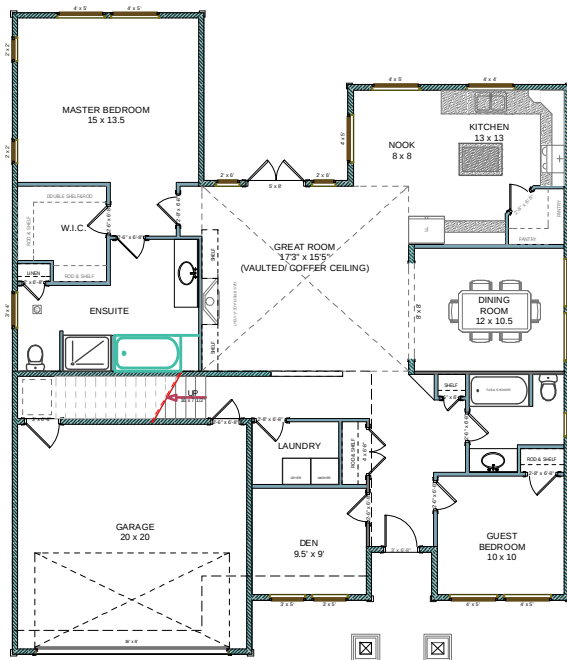
○ MAIN FLOOR PLAN (9'-0 3/4" WALLS) SCALE: 1/4" = 1' - 0" MAIN FLOOR AREA: 1,676 Sq Ft GARAGE AREA: 393 Sq Ft
