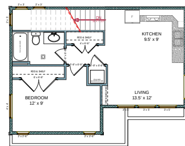
○ UPPER FLOOR PLAN (8'-0 3/4" WALLS) SCALE: 1/4" = 1' - 0" SUITE AREA: 520 Sq Ft
