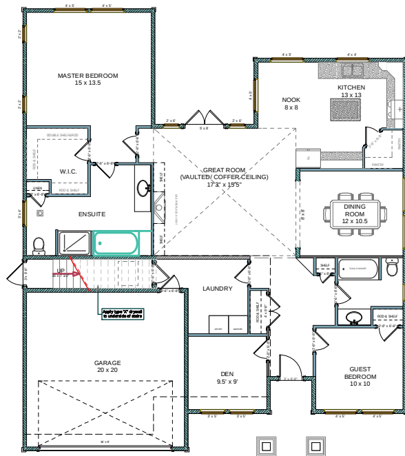
○ MAIN FLOOR PLAN (9'-0 3/4" WALLS) SCALE: 1/4" = 1' - 0" MAIN FLOOR AREA: 1,676 Sq Ft GARAGE AREA: 393 Sq Ft
